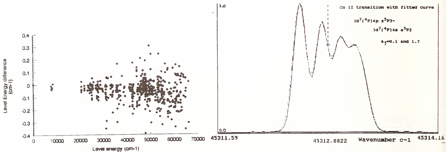
Fig.2 Cr level energy difference between this work and AEL[10]
